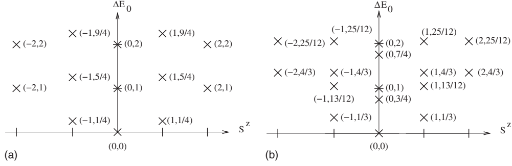
FIG. 8. The lowest excitations for \Delta=0 ( \Delta=1/2 ) in the left (right) panel. The energies corresponding to the crosses in the (S^z, \Delta E_0) plane are given in Eqs. (A1) and (A2), respectively.
